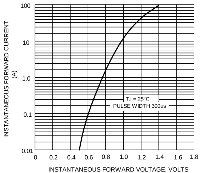
FIG.4-TYPICAL FORWARD CHARACTERISTICS
