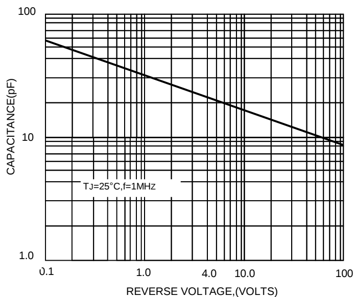
FIG.3-TYPICAL JUNCTION CAPACITANCE
